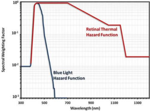
Figure 1: Retinal thermal and blue light hazard functions
